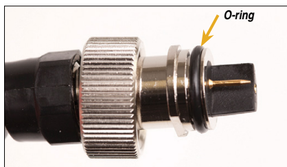
Lubricate O-ring for underwater operation.
