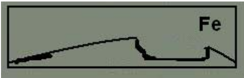
Big, deep, low magnetic ferrous target
